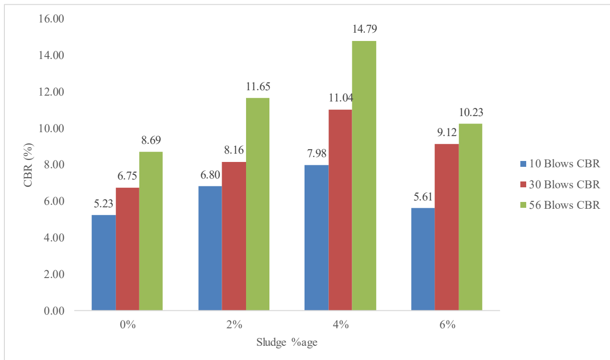
Figure 3 CBR % vs Sludge %age
